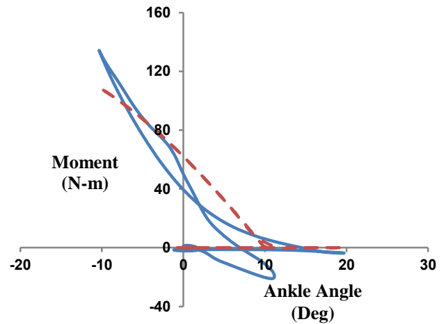
Figure 4. Human Ankle Work-Loops During Assisted Walking Calculated exoskeleton torque (N-m) (red/dashed curve) and ankle joint moment (N-m) (blue curve) versus ankle joint angle (deg) plotted over a full walking stride. The small inscribed area within the ankle joint work-loop (blue) indicates pseudo-spring-like behavior of the joint. To emulate these mechanics with our elastic exoskeleton we chose a spring and moment arm combination to generate torsional stiffness as close as possible to normal walking at 1.25 m/s. For both angles and moments + indicates plantarflexion/flexor.
