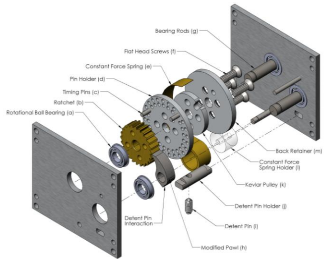
Figure 6. Exploded View of 'Smart-Clutch' Components Important features to note include: (b) ratchet (c) timing pins (h) pawl. Ankle joint movements are transmitted to rotation of the ratchet through the Kevlar and linear spring linkage over the stride. Timing pins are set to initiate and terminate engagement of the pawl at key points during
